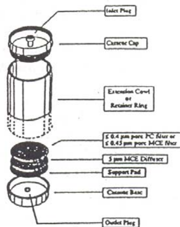
FIGURE 12-2 Air Sampling Cassette
